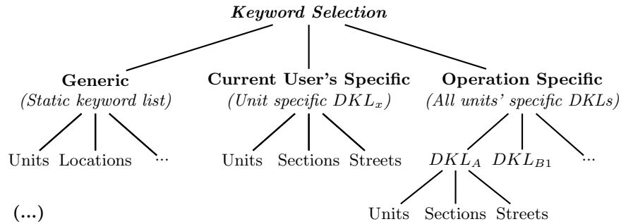
Figure 2. Example for clustering keywords for a guided keyword selection
