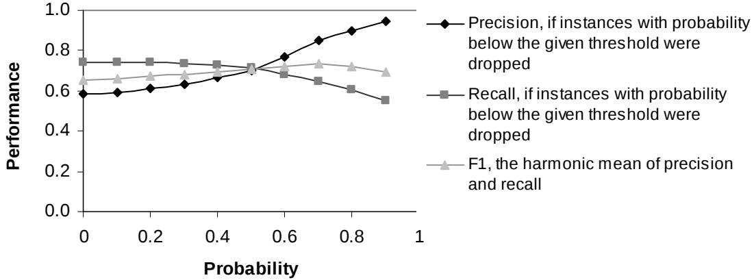
Figure 5. Precision, recall and F1 by PVotF for the domain of CS courses, regarding the threshold below which, the predicted instances are removed.
